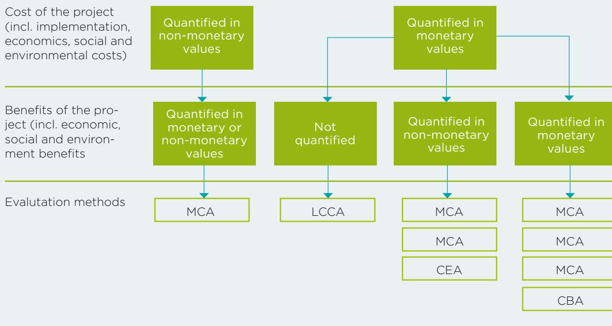
FIGURE 9.1 DECISION TREE
